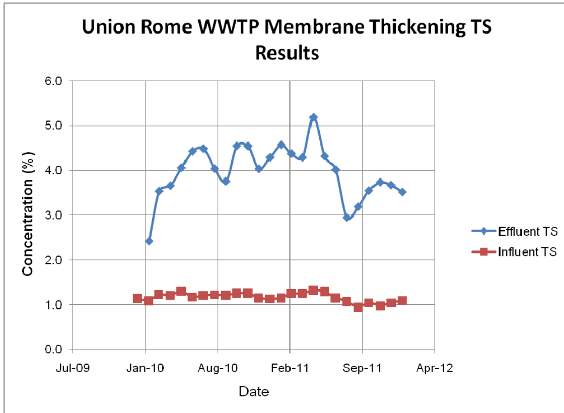
Figure 6. Union Rome WWTP Thickening Results of Aerobic Digestion System
