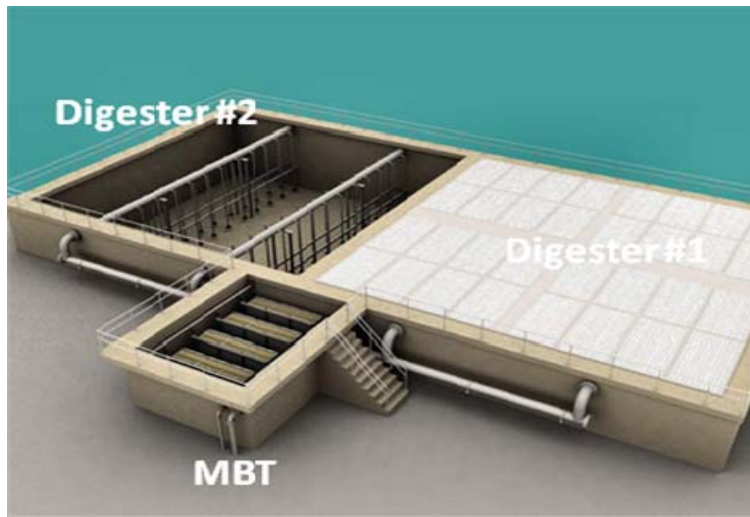
Figure 4: Dundee, MI WWTP Membrane Thickening Aerobic Digestion Facility
