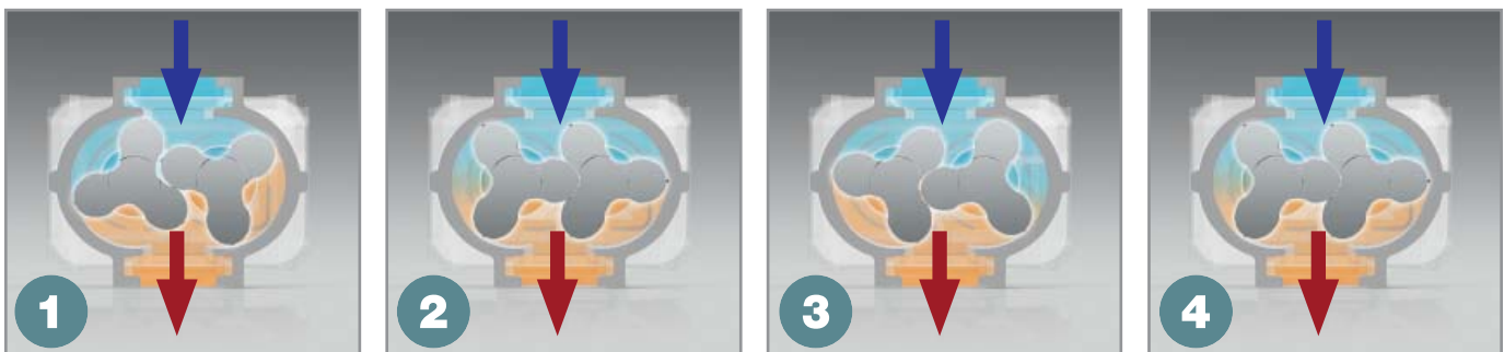
IMAGE 1: Pressure increasing — the images show the cross-section flow chamber of Kaeser’s rotary lobe blower block.
